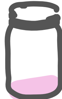
shoulder
