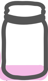
height
