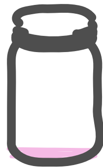
hair
